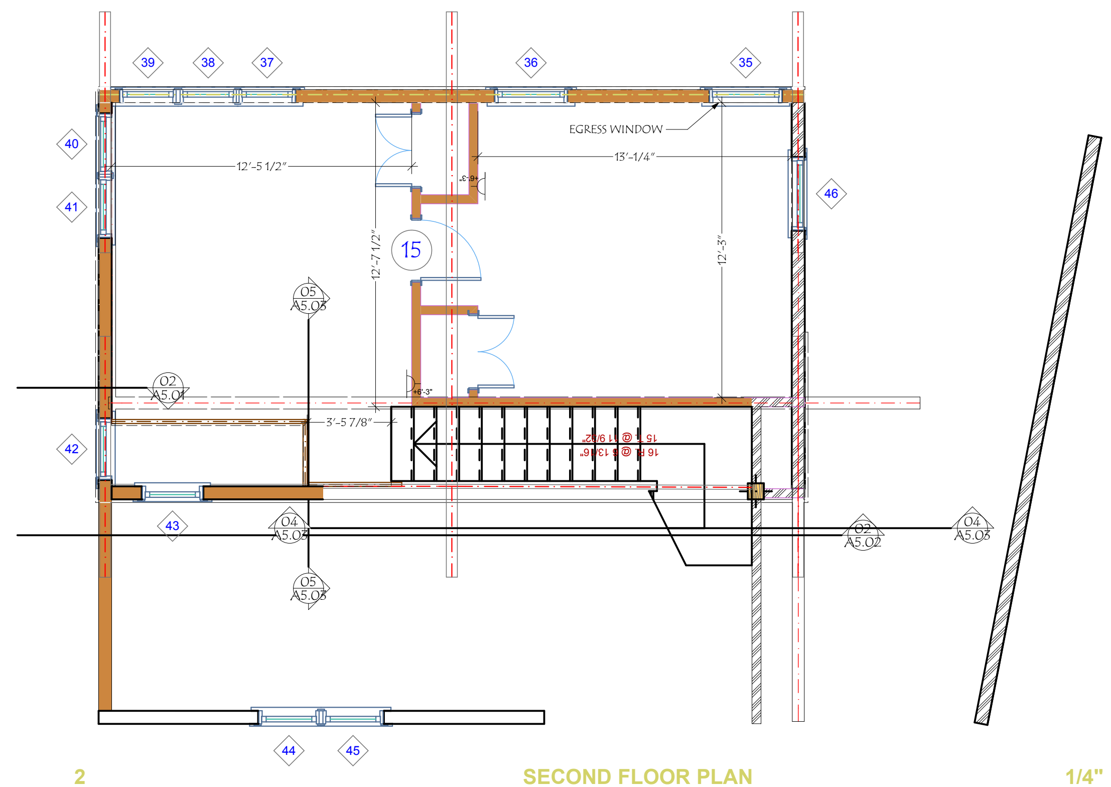
2 SECOND FLOOR PLAN 1/4" = 1'-0"
