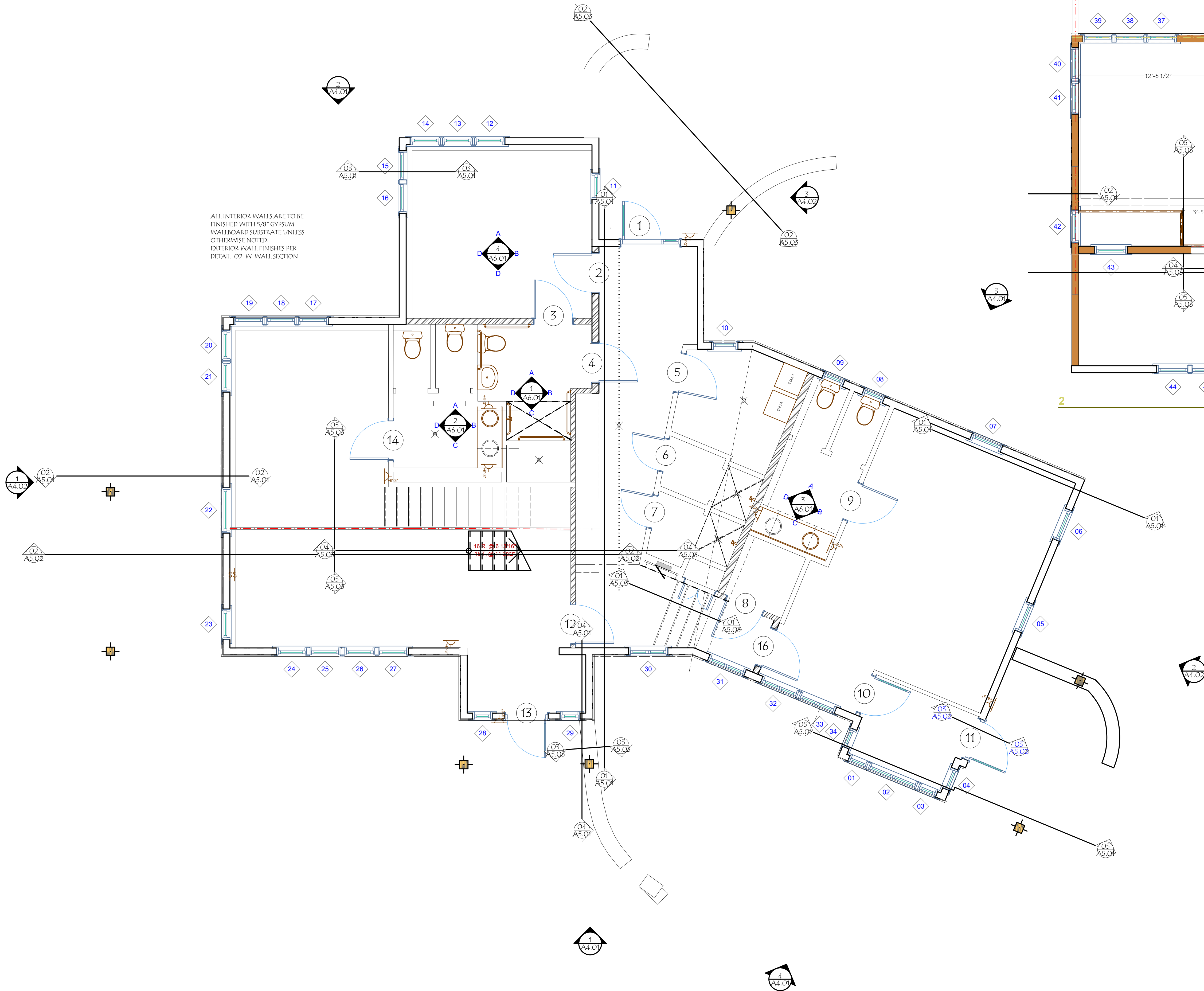
1 GROUND FLOOR PLAN 1/4" = 1'-0"
